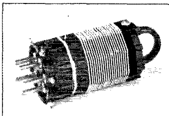
THE PILOT COIL FORM WITH THE 7000-KC. WINDING ON IT IS AT THE LEFT OF THE CONDENSER
