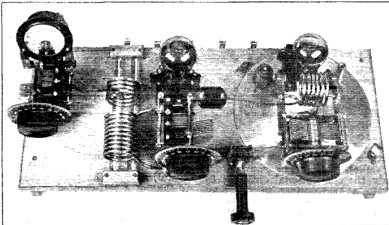
THE TRANSMITTER WITH THE OSCILLATOR SHIELD REMOVED
